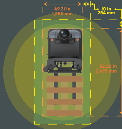
DRIVING SURFACE
